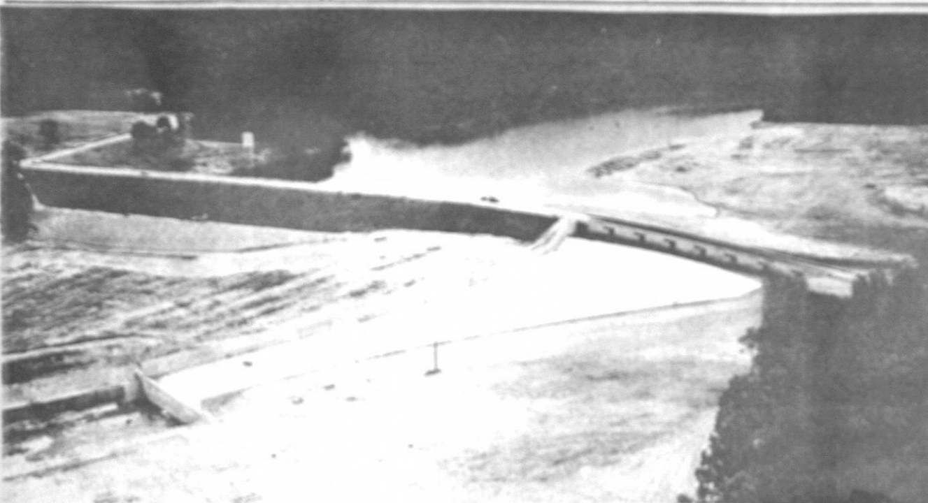
BEAR CREEK DAM —The new Bear Creek Dam, which TVA completed recently in Franklin County, Ala., is pictured above. The earthfill embankment is 1,400 feet long and 84 feet high. The concrete spillway is in the foreground and the water intake tower can be seen in the reservoir at the left. A road tops the dam and a concrete bridge spans the spillway. Fishing and boating are already being enjoyed on the 670 acre lake.
